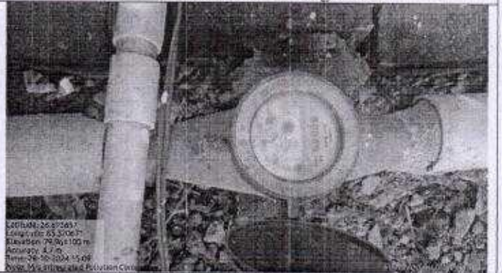
Flow Meter Installed at Inlet
