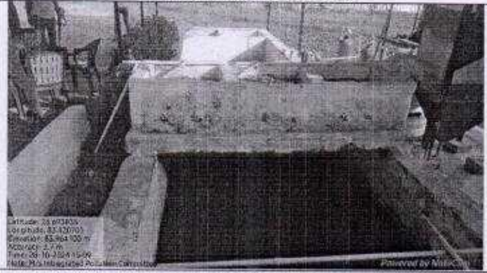
Sludge Drying Bed
